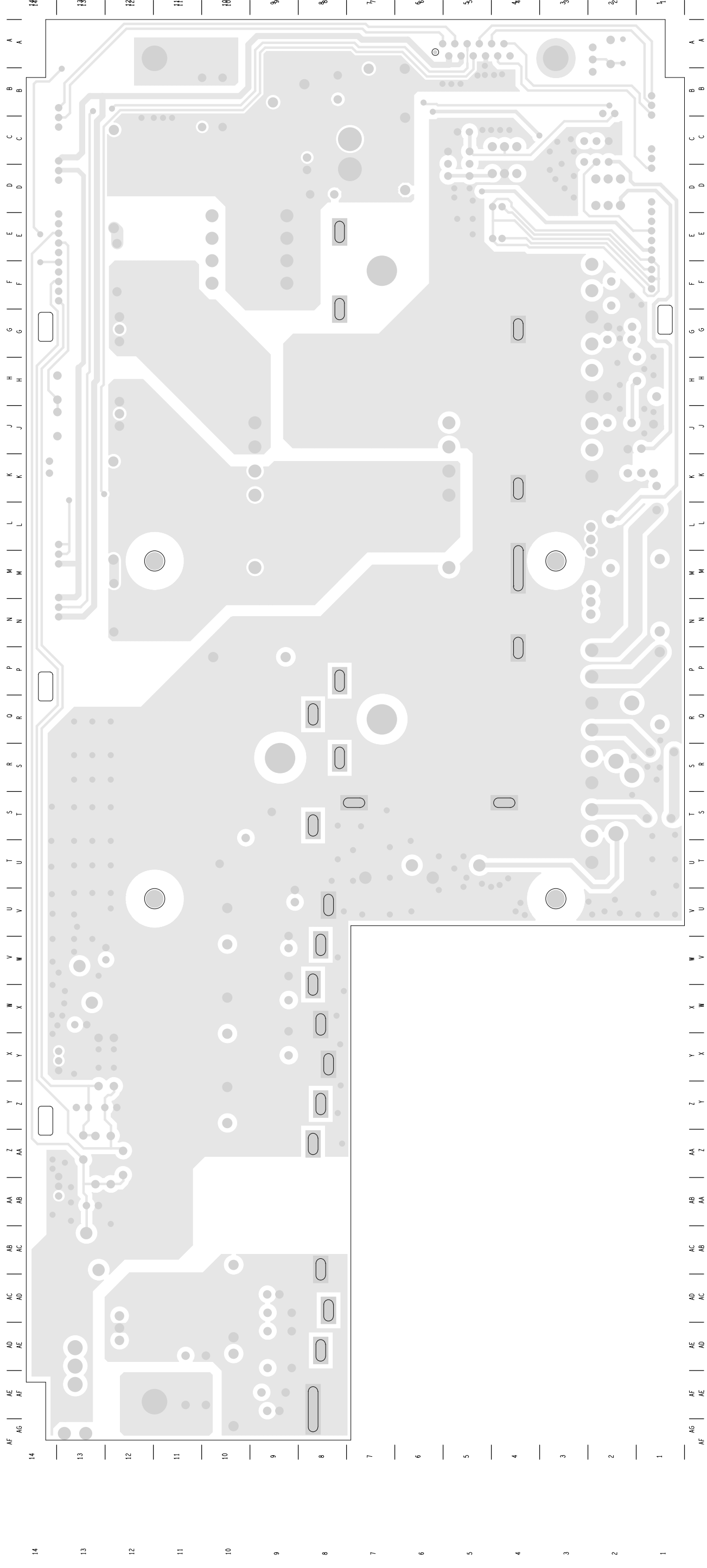
TAIT ELECTRONICS 1881 3038 3038 220-02012-07 A 300kg.05 NIS TB8000 DC-DC CONVERTER LAYOUT-SECONDARY-SIDE
